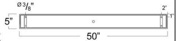
Canopy Mounting Detail Bottom view (Not to scale)
