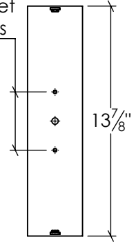
Backplate Mounting Detail Front View (Not to scale)
